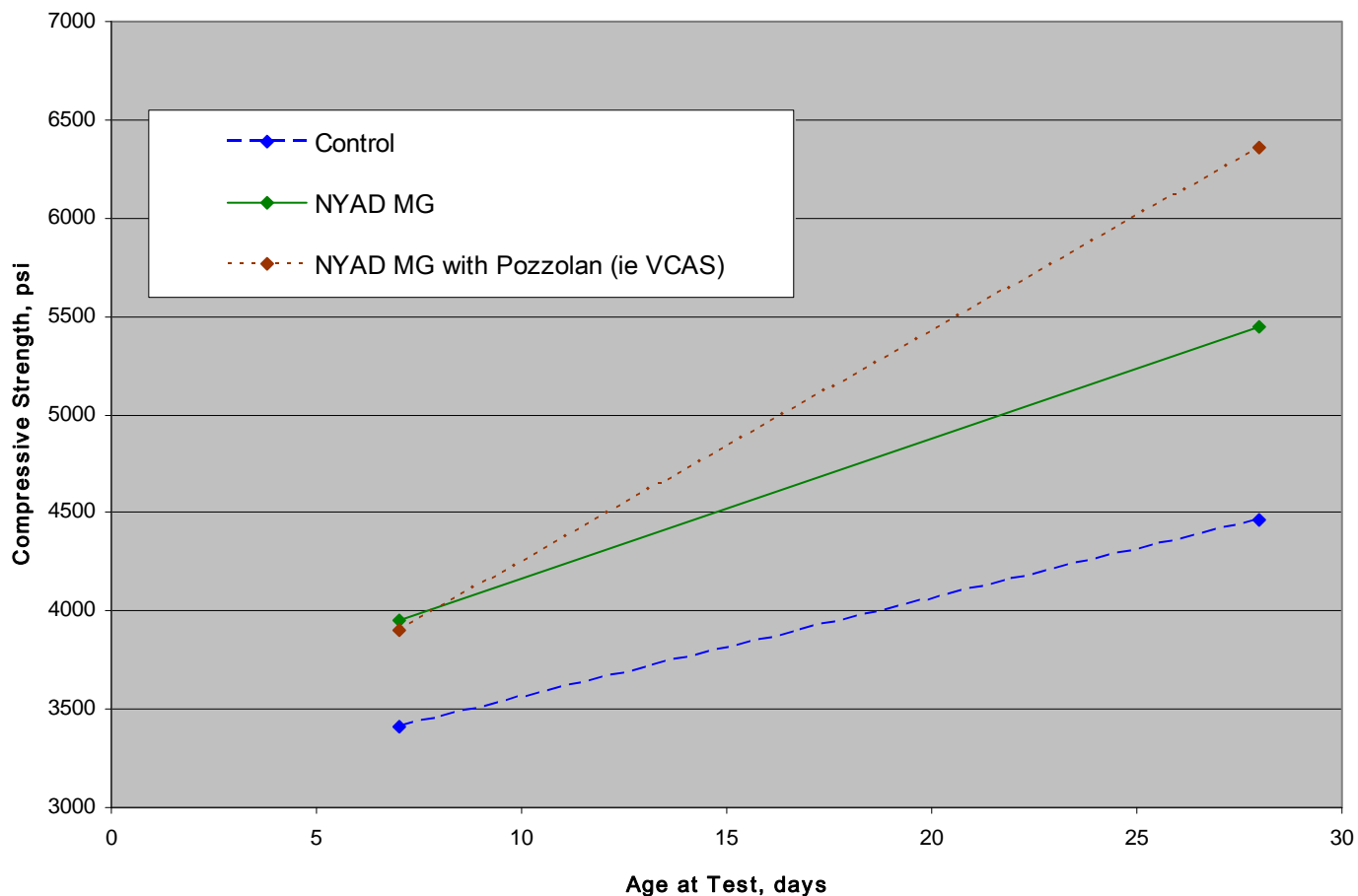
Compressive Strength Test Results (ASTM C 109)
